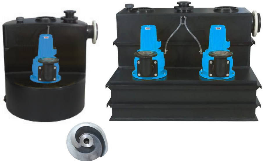
Channel Impeller
