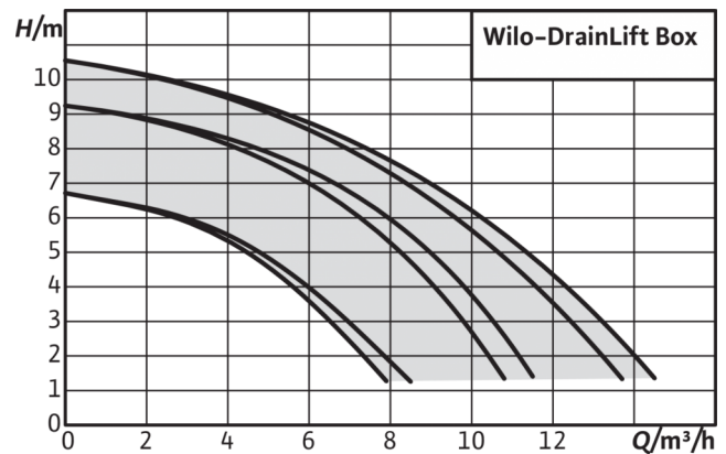
DrainLift Box
